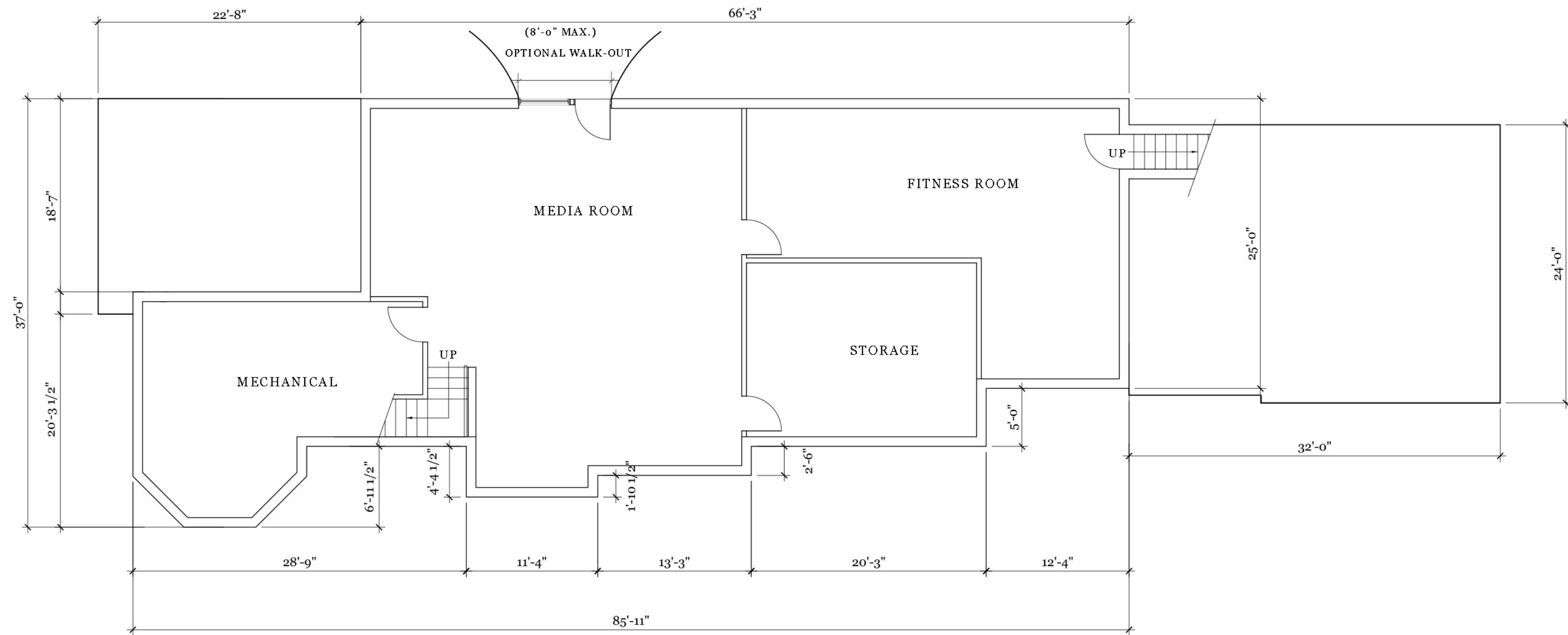
BASEMENT FLOOR PLAN
